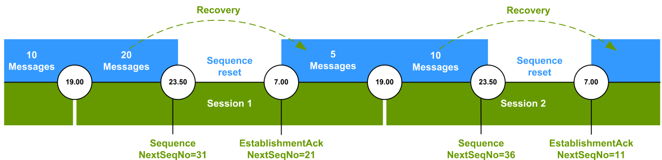
Figure 6. Diagram. Message counter reset
