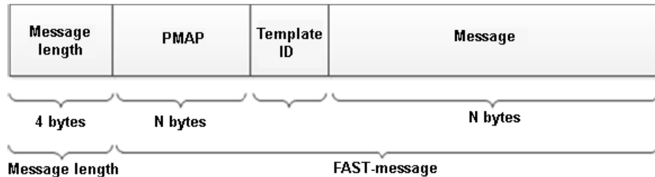
Pic. 2. Message structure in TCP stream
